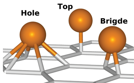
Figure 2. Possible adsorption sites for a single Fe atom inside a CNT as considered in ref.
